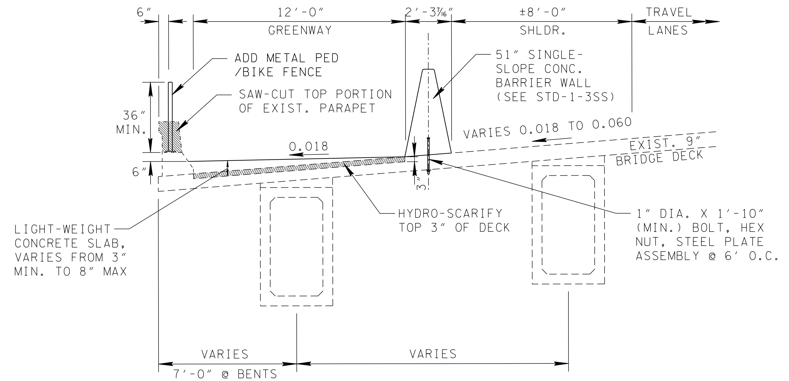
DETAIL PROPOSED GREENWAY ON BRIDGE
