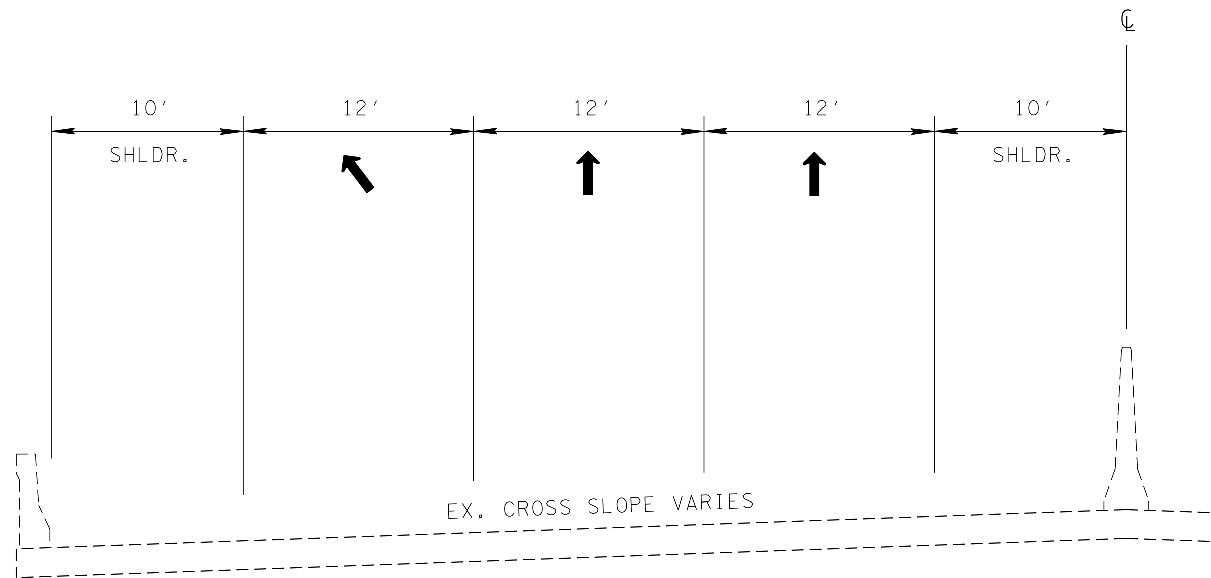
EXISTING BRIDGE JAMES WHITE PARKWAY STA. 19+12.69 TO STA. 38+20.75
