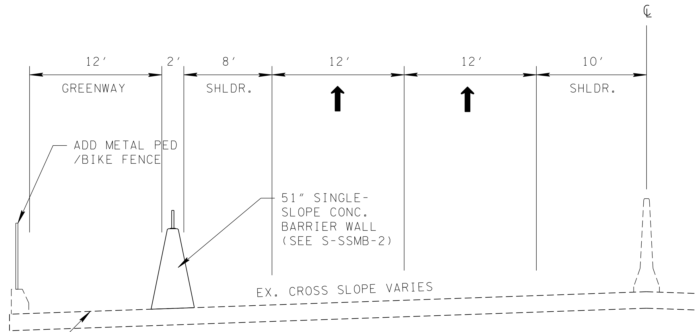
PROPOSED BRIDGE JAMES WHITE PARKWAY STA. 19+12.69 TO STA. 38+20.75
