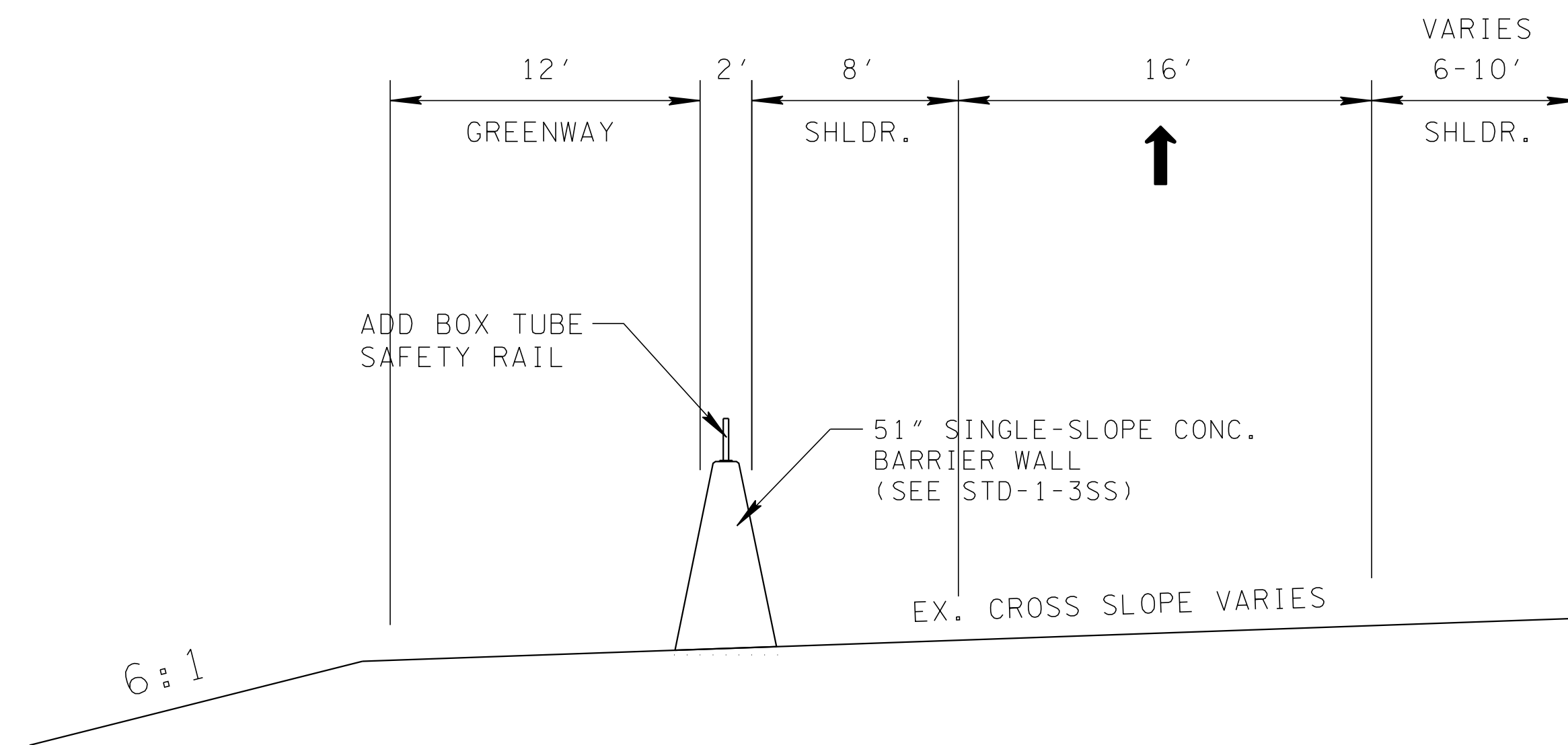
PROPOSED RAMP JAMES WHITE PARKWAY EXIT RAMP FROM ANITA DRIVE STA. 38+20.75 TO STA. 45+86.24
