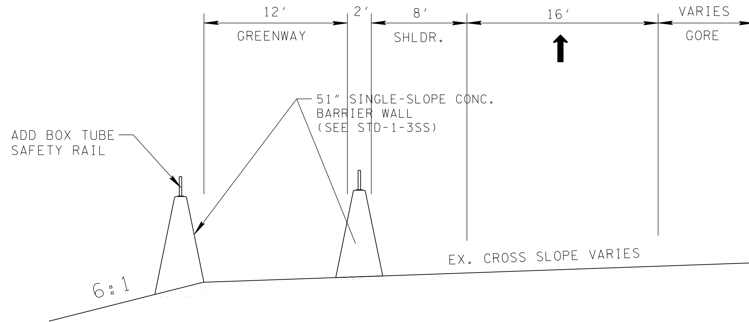
PROPOSED RAMP JAMES WHITE PARKWAY EXIT RAMP TO RIVERSIDE DRIVE STA. 10+05.31 TO STA. 19+12.69
